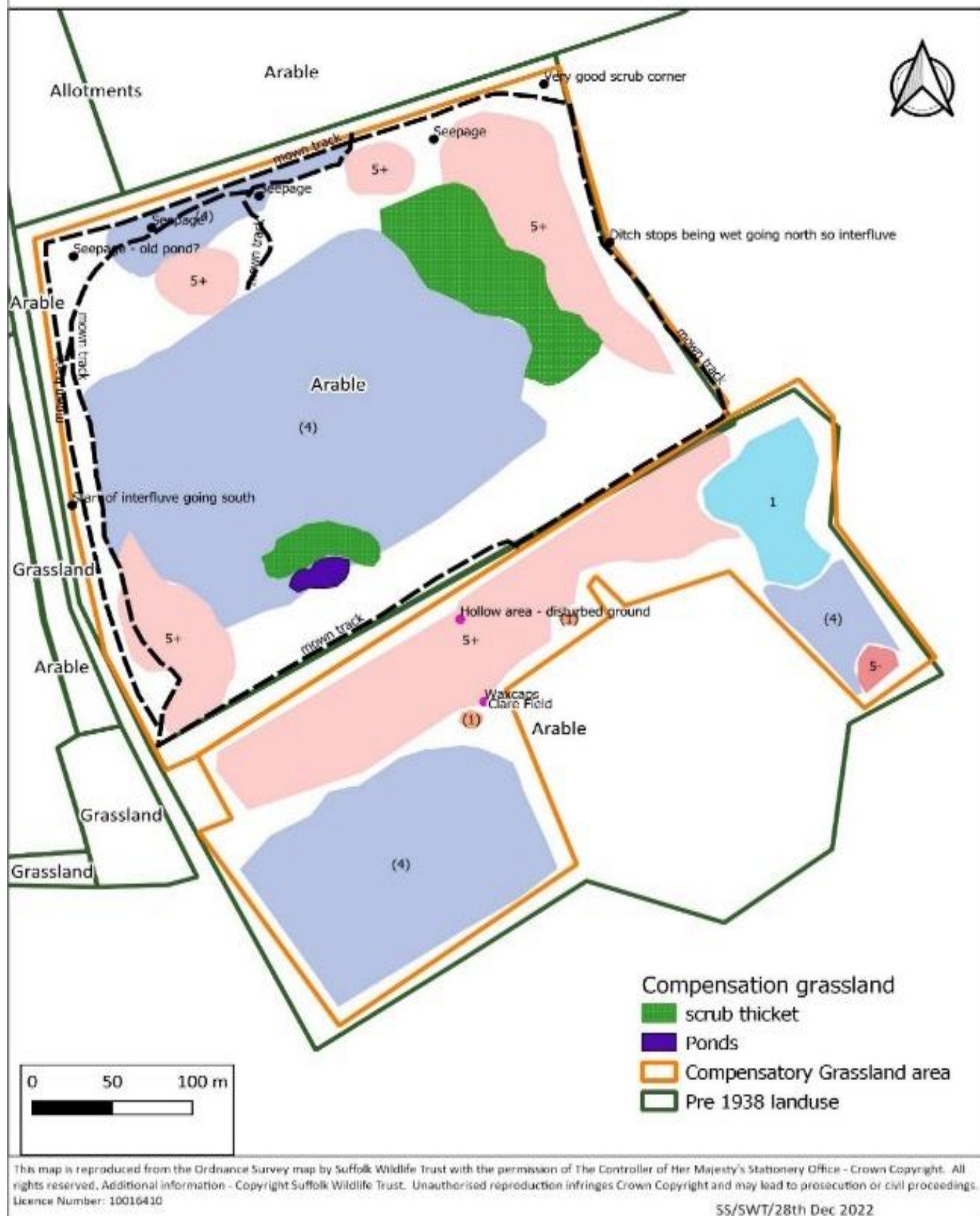
Figure 5: Overview of grassland types in Compensation Grassland (Management Plan Code D). Map taken from Broxted Solar Park Vegetation Monitoring Programme (Stone, 2022)
